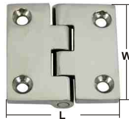
DOOR HINGE precision casted AISI 316 Reverse ITEM NO. WxLmm Thickness Weight/g 008511 50x50(2"x2") 4.5mm 89
