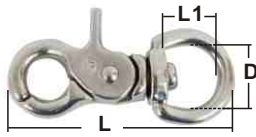
TRIGGER SNAP WITH SWIVEL EYE AISI 316 ITEM NO. L L1 D mm mm mm B19-034 46 12 14
