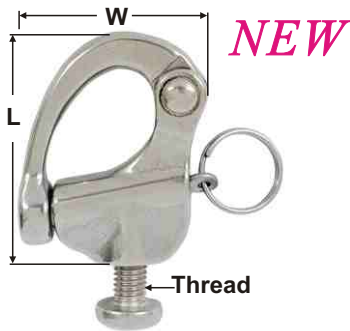
SNAP SHACKLE WITH SCREW AISI 316 (A4) ITEM NO. Thread L mm W mm Weight/g 004213 M6 40 35 40 004214 M8 52 46 90 004215 M10 72 57 270
