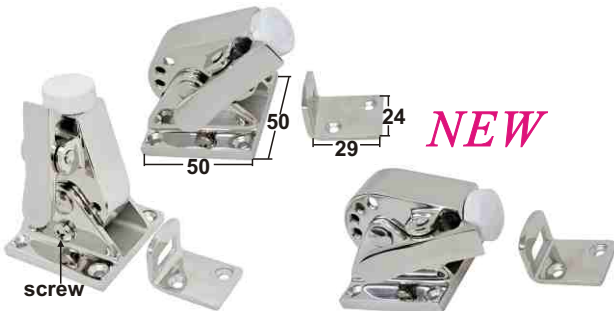
ADJUSTABLE DOOR HOLDER WITH FLUSH MOUNT PLATE AISI 316 Take off screw can adjustable angle ITEM NO. Base mm Weight/g B25-020 50x50 260
