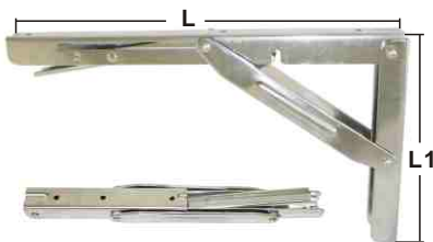
FOLDING BRACKET stamped AISI 304 For tales and working plates, Load up to 150kg ITEM NO. L L1 Weight/g 006133 303mm(12") 165mm(6-1/2") 530
