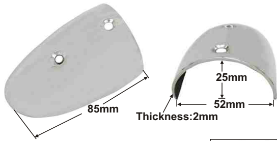
FENDER STRIP AISI 316 To mount on support PVC UV bases ITEM NO. B23-010
