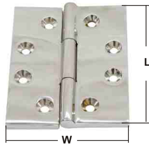
DOOR HINGE precision casted AISI 316 ITEM NO. WxLmm Thickness Weight/g 008515 80x100(3-3/16"x4") 4mm 300
