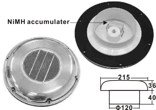
LOW PROFILE SOLAR VENTS WITH NIMH BATTERY stainless steel cover, stamped AISI 304 It needs rain or shine whether you're on the boat or not. solar cells power the fans for efficient, active ventilation. Low profile. Single crystal solar cells recharge NiMH battery for 24 hours operation. ITEM NO. Basement Weight/g 003794 215mm(8-1/2") 800
