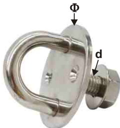
EYE PLATE with WASHER & NUT stamped AISI 304 ITEM NO. \Phi mm Thickness d mm Weight/g 003590 33 2.5mm M6 28 003591 40 2.5mm M8 50 003592 50 3.0mm M10 90
