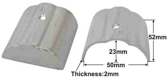
FENDER STRIP AISI 316 To mount on support PVC UV bases ITEM NO. B23-022
