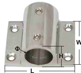
TUBE HOLDER casted AISI 316 ITEM NO. For tube \Phi L mm W mm H mm Weight B19-019 22 mm 58 46 29 160g B19-020 25 mm 61.5 46 33 180g
