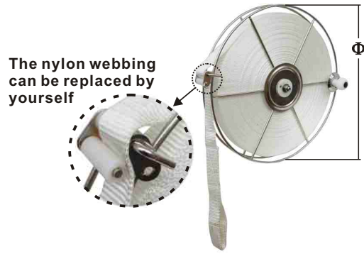
STERN ANCHOR ROLLER AISI 304 mounting for \Phi 22mm & 25mm rail tube with belt
