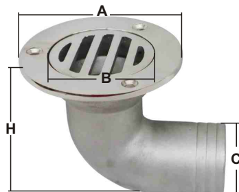
SHOW / COCKPIT DRAINERS stainless steel AISI 316 ITEM NO. Flange Φ(A) Application hole (B) Hose adaptor (C) H mm Weight/g B19-018 80 mm 50 mm 38 mm 70 380
