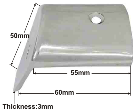
FENDER STRIP AISI 316 To mount on support PVC UV bases ITEM NO. B23-024
