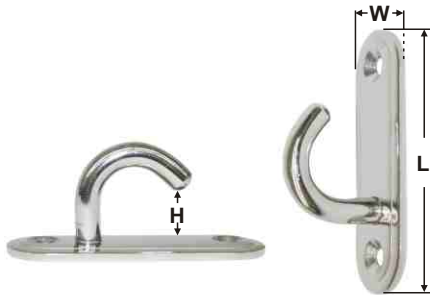
PLATE HOOK stamped AISI 304 ITEM NO. L mm W mm H mm Weight/g 003597 45(1-49/64") 15(5/8") 9 15 003598 60(2-23/64") 20(25/32") 13 30 003599 80(3-5/32") 25(1") 15 60
