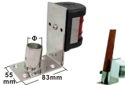
FLAG AND NAVIGATION LIGHT SOCKETS AISI 304 (Less navigation light) ITEM NO. Φmm Weight B18-018 25 190g
