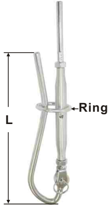
FORESTAY TENSIONNER WITH RING AISI 304 Not include turnbuckle & swadge terminal ITEM NO. L mm Ring \Phi mm(inside) Wire \Phi mm 004900 115 30 6 004901 105 33 8 004902 220 40 10 004903 260 46 12
