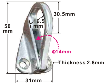
FENDER HOOK WITH SAFTY SNAP AISI 316 ITEM NO. B23-009
