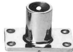
90° RECTANGULAR BASE casted AISI 316 ITEM NO. Tube O.D. Base mm Weight/g 009678 32mm(1-1/4") 82x42 250
