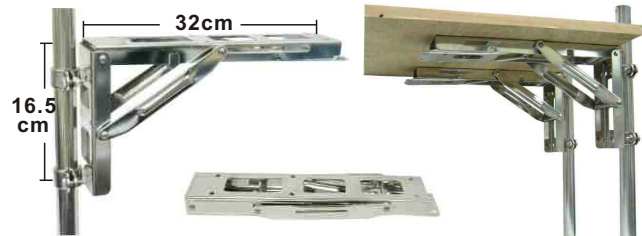
BRACKET ASSEMBLY stainless steel Folding bracket for table and working plates. Very stable, load up to 150kg. the set consists of 2 brackets, 4 clips (22-25mm tube) and 4 screw with nuts. ITEM NO. 006131
