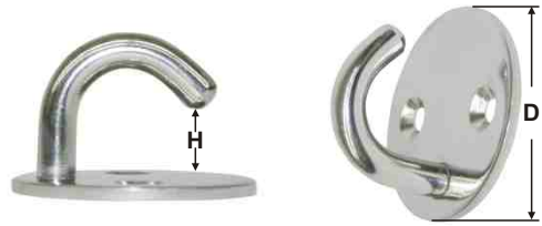
ROUND PLATE HOOKS stamped AISI 304 ITEM NO. D mm H mm Thickness Weight/g 003695 33 9 2.5mm 20 003696 40 9 2.5mm 40 003697 50 15 3.0mm 60
