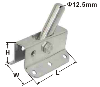
MAST FITTING Stamped AISI 304 ITEM NO. L H W mm mm mm Weight/g B17-009 65 35 42 140
