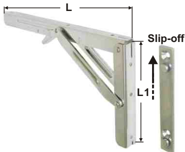
SLIP-OFF FOLDABLE ARMS stamped AISI 304 For table can be slipped off their wall support. Load up to 150kg ITEM NO. L L1 Weight/g 006135 303mm(12") 165mm(6-1/2") 650
