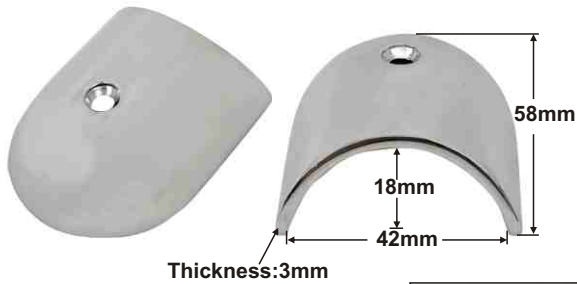
FENDER STRIP AISI 316 To mount on support PVC UV bases ITEM NO. B23-020
