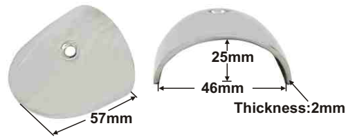
FENDER STRIP AISI 316 To mount on support PVC UV bases ITEM NO. B23-011
