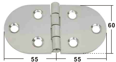
HINGE stamped AISI 304 ITEM NO. Thickness Weight/g 008513 2mm 95
