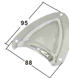
VENT AISI 304 ITEM NO. LxWxHmm Type Weight/g 003751 95x88x24 midget 50
