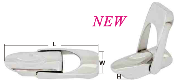
STAINLESS STEEL LEVER CLOSURE FOR TIGHTLY CLOSING HATCHES AISI 316 Lever lock made of highly polished AISI 316, which is suitable for various applications and securely closes any storage box. When the closure is open, the closure hook rotates 180° so that it cannot be accidentally bumped. ITEM NO. L mm W mm H mm Weight/g B25-012 81 26 11 60
