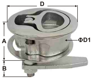
LIFTING HANDLE AISI 316 ITEM NO. D mm D1 mm A mm B mm weight/g B22-010 61 51 21 39 280
