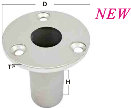
TARP TUBE HOLDER COUNTER SUNK AISI 316 ITEM NO. For tube \Phi mm D mm H mm T mm Weight/g B25-016 20 63.5 64 4 210 B25-017 22 63.5 64 4 200 B25-018 25 70 64 4 300 B25-019 30 70 64 4 310
