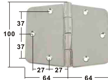
HINGE stamped AISI 316 buff polished ITEM NO. Thickness Weight/g 006132 3mm 340
